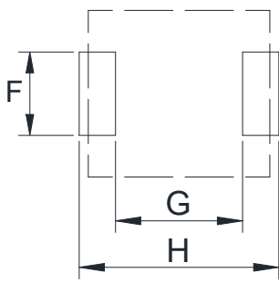
Reference PCB pattern
